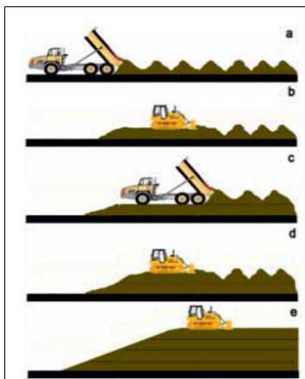
Figure 4-2: Stockpile formation from dry soils
