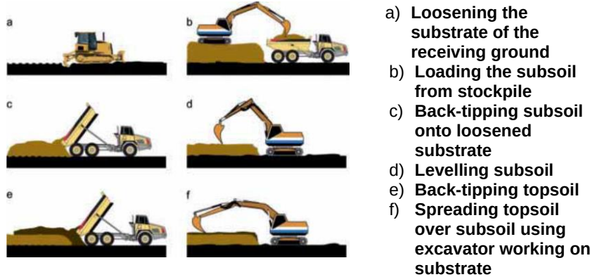
Figure 4-6: Loose-tipping method for subsoil and topsoil placement
