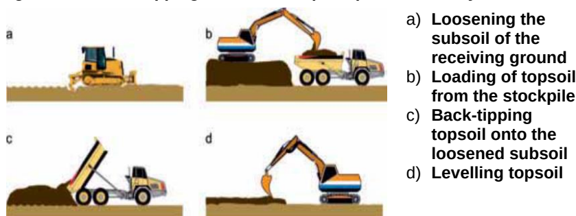
Figure 4-5: Loose-tipping method for topsoil placement only
